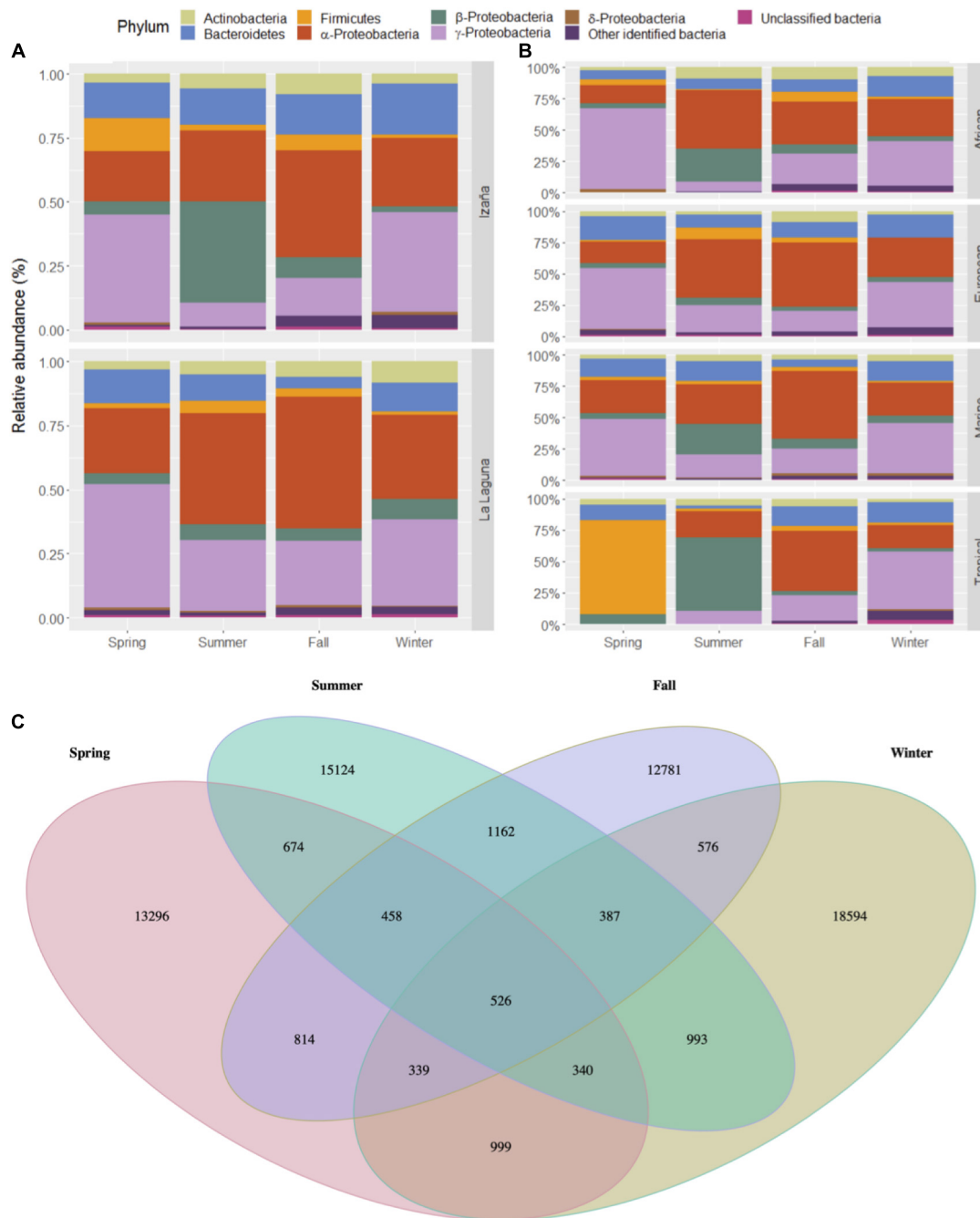
FIGURE 3 | Relative abundances of the most predominant bacterial taxa at the phylum level in both locations by season (A) and wind back trajectory (B). Venn diagram of unique and common bacterial phyla by season (C).
